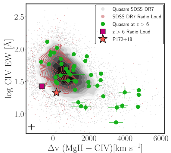
Figure 4. C IV equivalent width vs. blueshift with respect to the Mg II emission line. We show the distribution of SDSS DR7 1.4 < z < 2.2 quasars with gray points and shaded gray contours. The radio-loud subsample from SDSS is highlighted with red points and contours (see Section 3.1 for definition and selection). Quasars at z > 6 are reported with green points, and obtained from a collection of works from the literature (Mazzucchelli et al. 2017, Shen et al. 2019, Onoue et al. 2020, Schindler et al. 2020). Before this work, there was only one z > 6 radio-loud quasar with robust C IV and Mg II measurements (magenta square). P172+18 at z = 6.823 is represented as an orange star and its uncertainties are shown in the bottom left corner.
