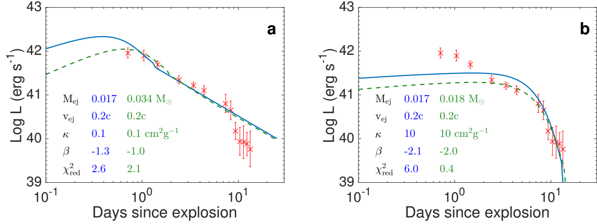
Figure 3: | Model light curve fits using the Arnett formalism. Mass, velocity, opacity ( \kappa ) and a power-law slope for radioactive powering ( \beta ) are freely variable. Each of these parameters were allowed to vary to give the best fit (reduced \chi^2 are quoted). a: The blue solid line shows the best fit. The green dashed model includes also a thermalization efficiency 19 . The recovered power law ( \beta = -1.0 to -1.3 ) is close to the one predicted in kilonova radioactivity models ( \beta = -1.2 ). b: Best fits when opacity is forced to \kappa = 10 \text{ cm}^2 \text{ g}^{-1} , to all data (blue, solid) and excluding first three data points (green, dashed). In all models the maximum allowed velocity is 0.2c , which is also the preferred fit value. The errors are 1\sigma uncertainties on the data, while the later points after 10 days are uncertain due to systematic effects. The full MCMC analysis and uncertainties are discussed in the Methods section.
