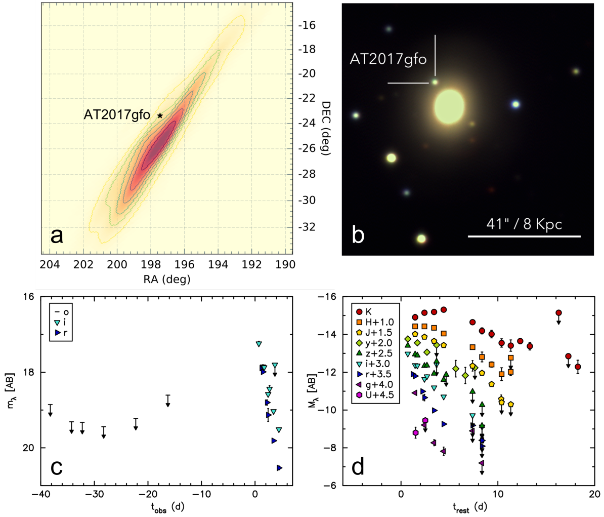
Figure 1: | Observational data summary a: The position of AT2017gfo lying within the Ligo-Virgo skymap 11,6 b: Color composite image of AT2017gfo from GROND on 20170818 (MJD 57983.997), 1.45 days after GW170817 discovery. The transient is 8.50'' North, 5.40'' East of the centre of NGC4993, an S0 galaxy at a distance of 40 \pm 4 Mpc. This is a projected distance of 2 kpc. The source is measured at position of RA=13:09:48.08 DEC=-23:22:53.2 J2000 ( \pm 0.1'' in each) in our Pan-STARRS1 images. c: ATLAS limits between 40 and 16 days before discovery (orange filter), plus the Pan-STARRS1 and GROND r and i -band light curve. d: Our full light curve data, which provides a reliable bolometric light curve for analysis. Upper limits are 3\sigma and uncertainties on the measured points are 1\sigma .
