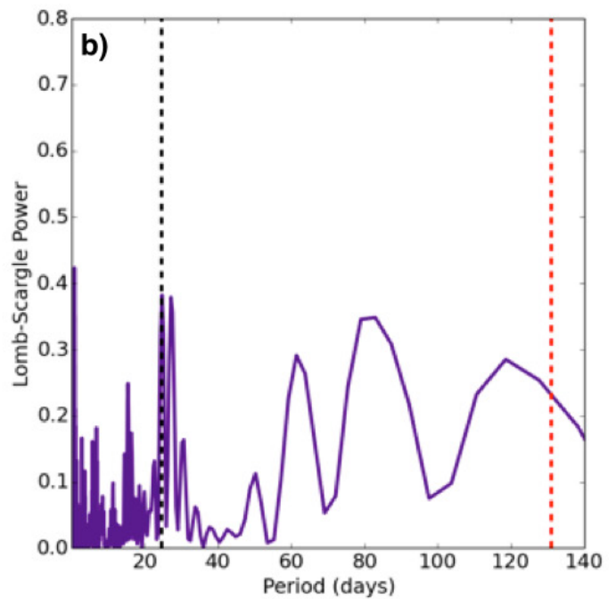
b , Periodogram for our HARPS radial-velocity observations. We see substantial power near the 24.73712-day orbital period of LHS 1140b (black dashed line), as well as broad power at longer periods associated with stellar rotation (131 days, red dashed line) and at shorter periods associated with the window function of our observations.
