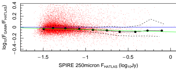
Figure 20. A comparison between the preliminary Herschel-ATLAS 5\sigma catalogue and the optically motivated catalogue derived here in the SPIRE 250\mu\text{m} band. It should be noted that the zero-points calibration and entire reduction process have evolved between these catalogues. Note units are in Jansky as is standard in the far-IR.
