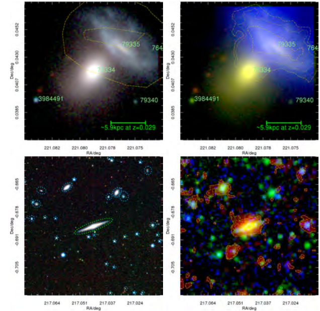
Figure 15. Upper left: A colour composite image of G79334 produced by combining the SDSS g & r with the VIKING H band images. Overlaid are the contours from SPIRE-250 band. GAMA IDs are marked. Upper right: A colour composite of G79334 from GALEX NUV, VIKING Z & K_s and with contours overlaid from WISE. Lower left: A 2' \times 2' colour composite centred on G48432 made from data extracted from the GAMA SDSS r & i SWarp combined with the VIKING H SWarp and with the apertures used for the aperture-matched photometry overlaid. (lower right) A composite colour image of G48432 made from GALEX FUV (blue channel), WISE W1 (green channel) and SPIRE 250\mu\text{m} (red channel and contours). All images produced using the online GAMA \Psi tool: http://gama-psi.icrar.org/
