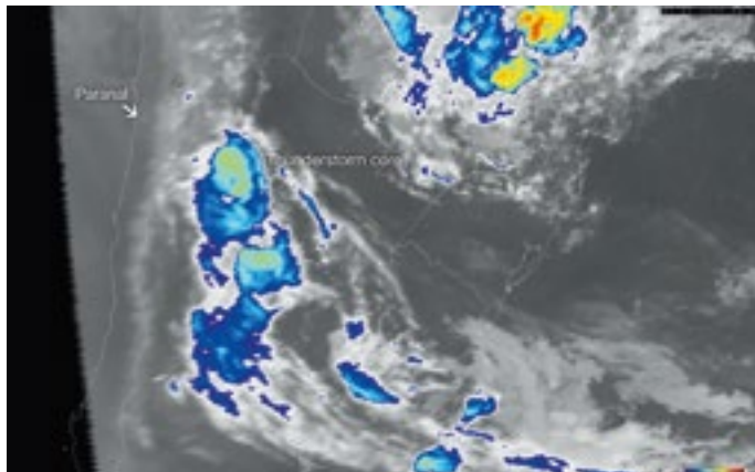
Figure 4. Image taken by the Meteosat-10 satellite on 27 January 2015 at 8:45 UTC as the thunderstorm's activity decreased. The weakening storm cell, above which the sprites in Figure 3 were observed, is indicated.
