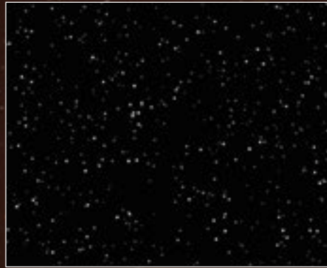
Distant/Early galaxies seen by ALMA (simulated)
