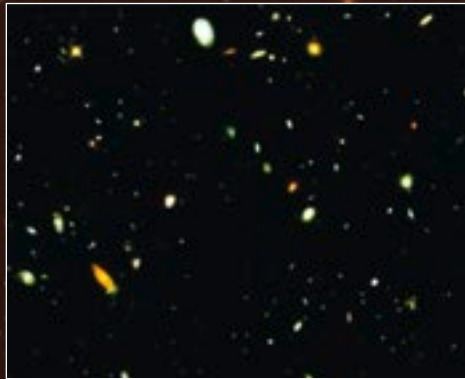
"Nearby" galaxies seen by Hubble
