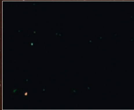
Distant/early galaxies seen by Hubble
