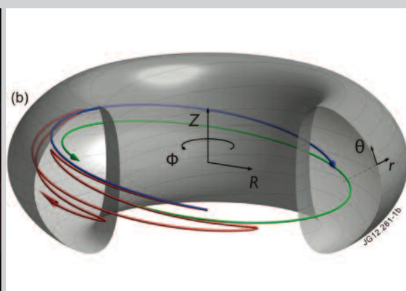
Illustration of magnetically trapped particle trajectories in the earth's magnetosphere (a), and magnetically confined particle trajectories in a tokamak fusion reactor (b).
