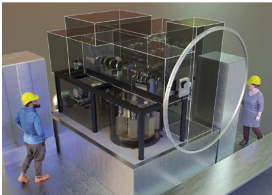
Computer rendering of MAVIS on the instrument platform of VLT Unit Telescope 4. The boxes indicate the various submodules of the instrument.
