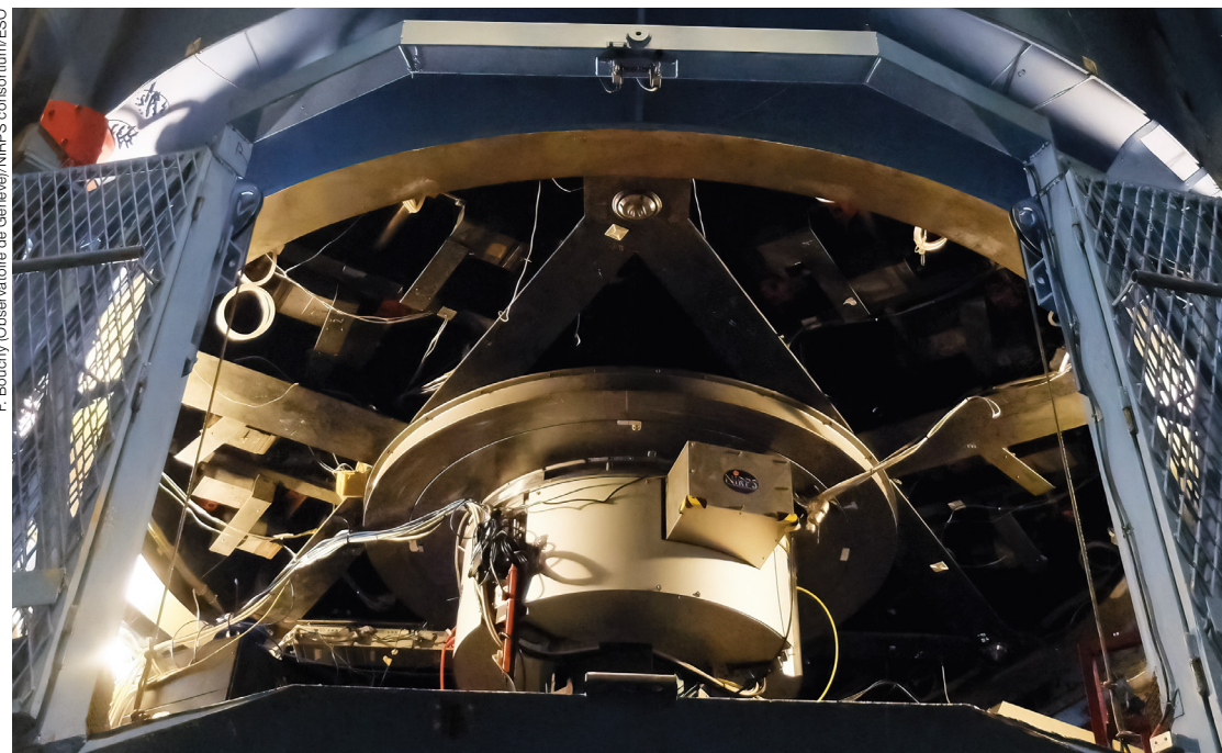
The front end of the NIRPS (Near Infra-red Planet Searcher) instrument, including its adaptive optics system, sits just under the primary mirror of ESO's 3.6-metre telescope.
