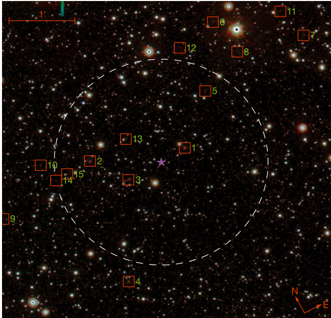
VISTA image of a cluster of galaxies behind the Galactic Plane. The circle indicates the X-ray position of the cluster. Individual cluster galaxies are shown in the postage stamps. From Coldwell et al. (2014).
