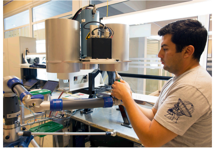
An amplitude calibration device being serviced at the OSF. Each ALMA antenna has one of these devices to calibrate of the radio signals.
