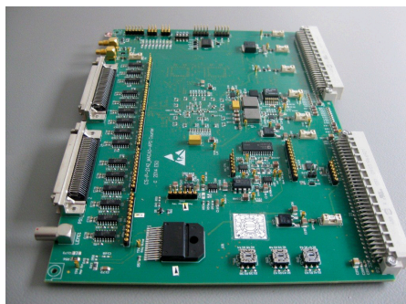
Replacement avalanche photodiode board for NACO, based on field-programmable gate array technologies.
