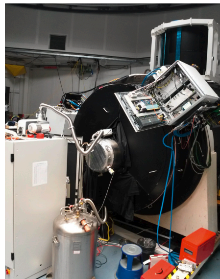
The AOF test configuration in the Garching laboratory: the deformable secondary mirror sits on top of the ASSIST bench and the GRAAL module is mounted on the Nasmyth focus simulator, with the CAMCAO silver cryostat in the foreground.
