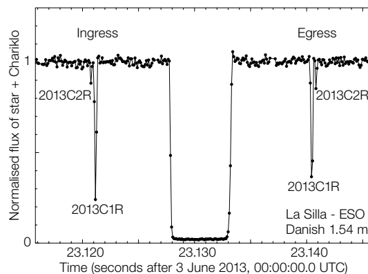
Light curve of the occultation by the Chariklo system taken on 3 June 2013 with the Danish 1.5-metre telescope. The central dip is caused by the occultation by Chariklo of the star, whilst the two secondary events 2013C1R and 2013C2R are attributed to the ring system. From Braga-Ribas et al. (2014).
