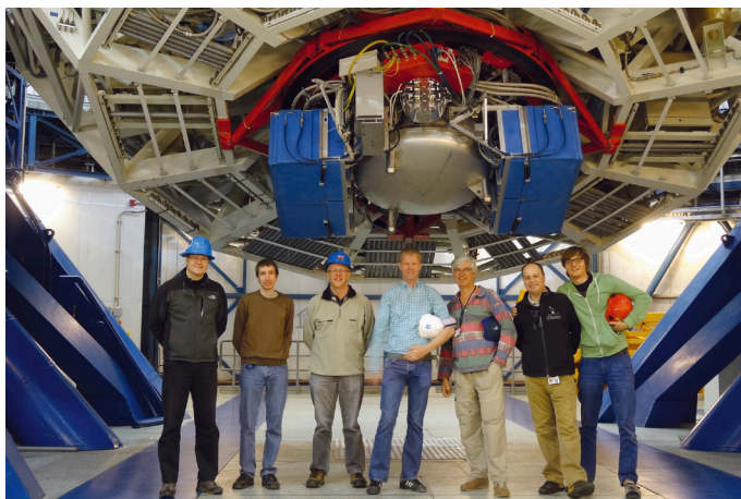
VISIR re-commissioned at the Cassegrain focus of UT3.
