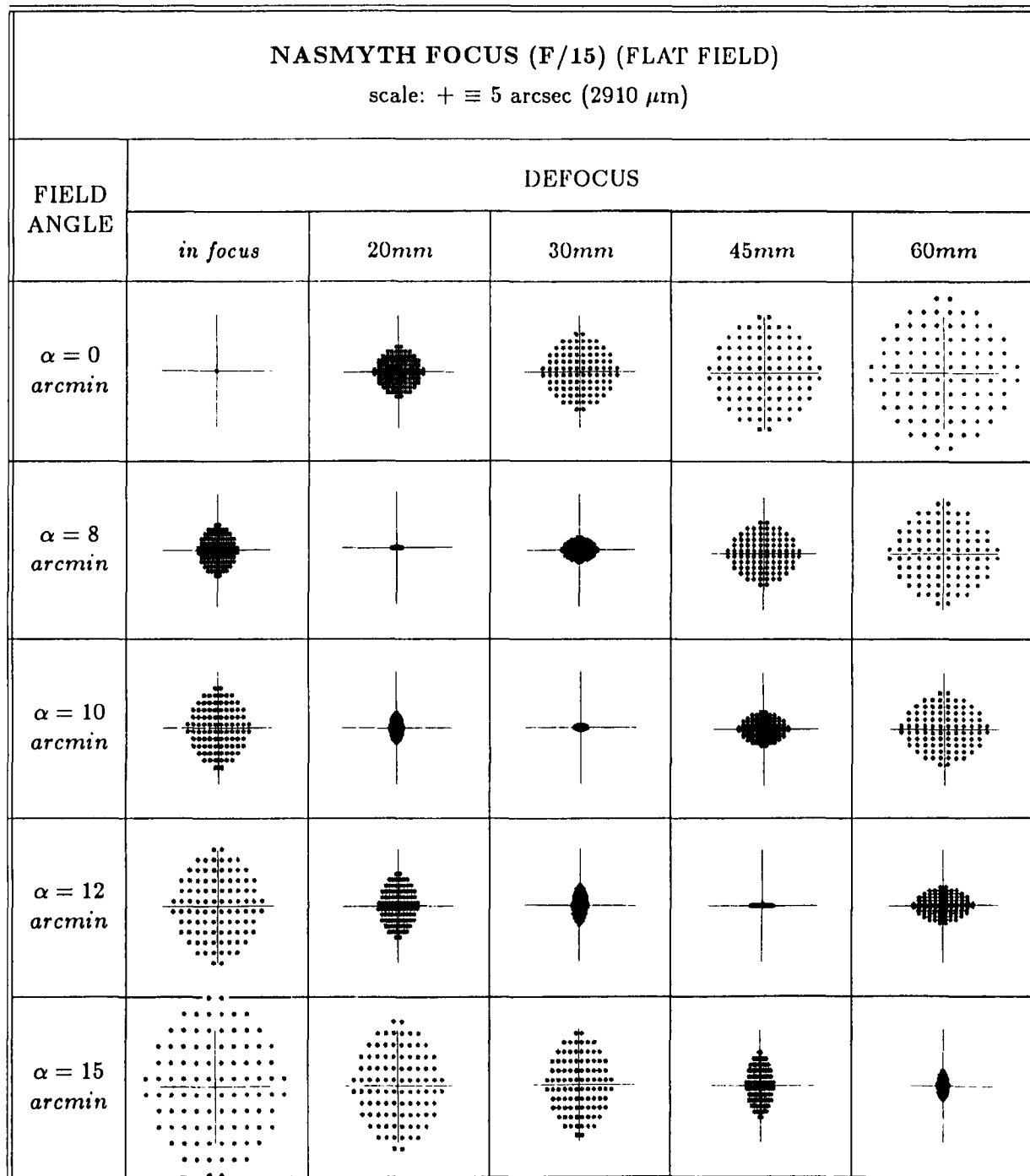
Figure 4.4: Spot diagrams for a flat field at a Nasmyth focus of the VLT unit telescope.
