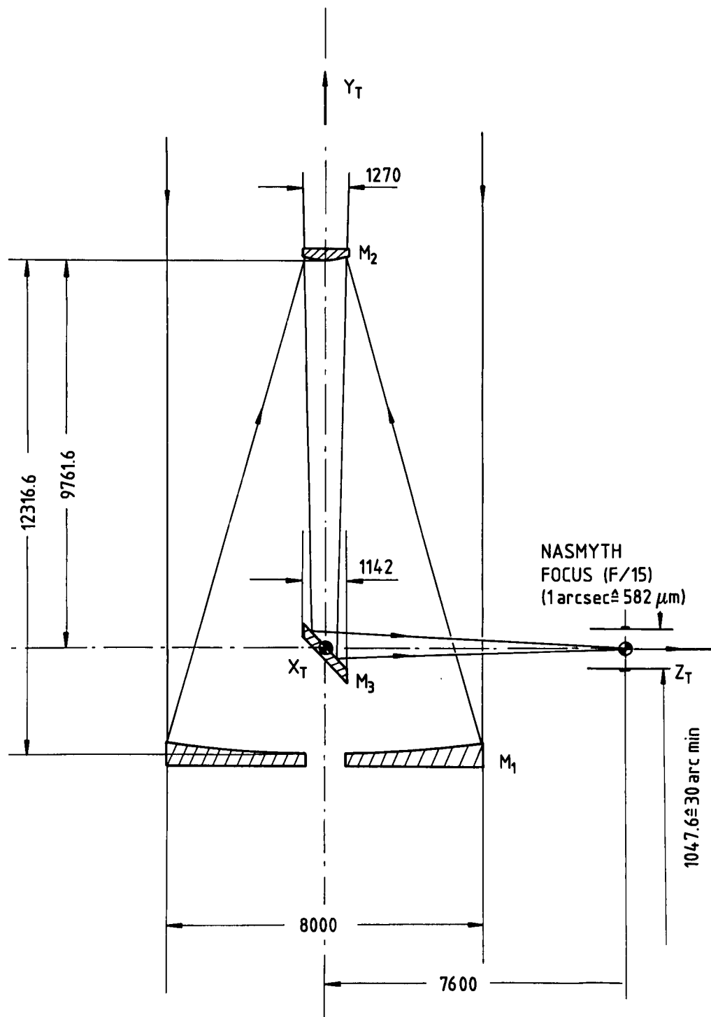
Figure 4.2: Optical design of the 8m unit standard telescope with Nasmyth focus. M_3 is rotated around the Y -axis for the second Nasmyth focus.
