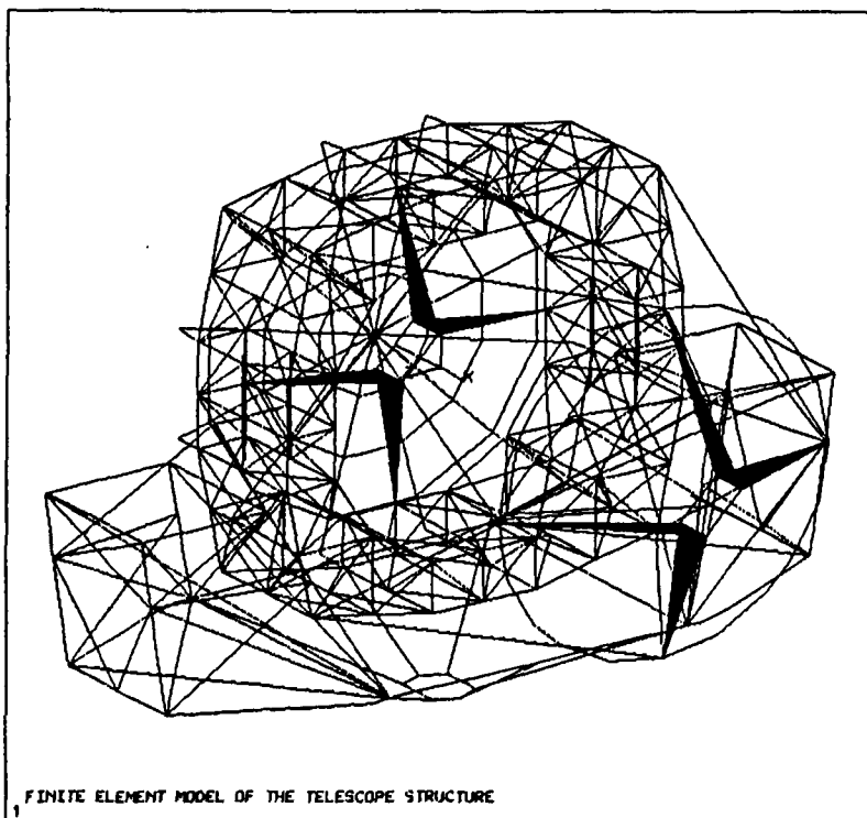
Figure 6.5: Finite element model of telescope structure.
