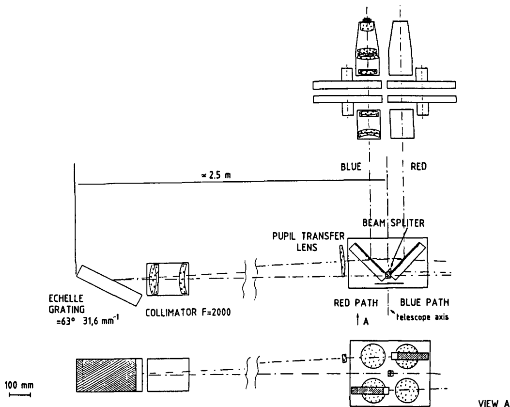
Figure 10.5: A preliminary layout of a multimode instrument for the Nasmyth focus of the VLT. In the medium resolution mode ( R = 15000 ) the field slicer which feeds the array of focal reducers of the EFOSC type is replaced by a slit and a dichroic beam splitter. The red and blue arms mount double-pass collimators and echelle gratings. The spectra are finally reimaged on the detectors through two EFOSC channels. Cross dispersion is provided by grisms. The medium dispersion arms are stationary and the instrument will work on axis in that mode.
