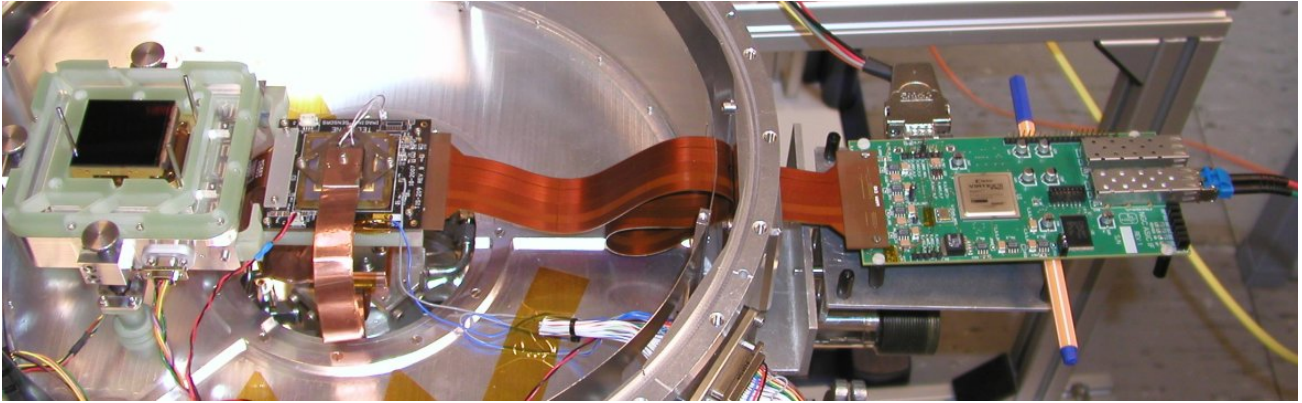
Figure 4 Cryogenic setup with ASIC and HyViSI FPA in the ESO test cryostat.
