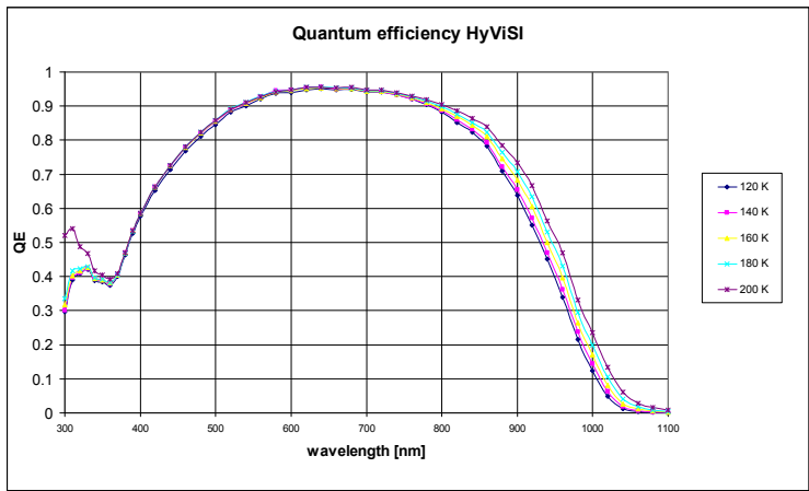
Figure 6 HyViSI QE at various temperatures
