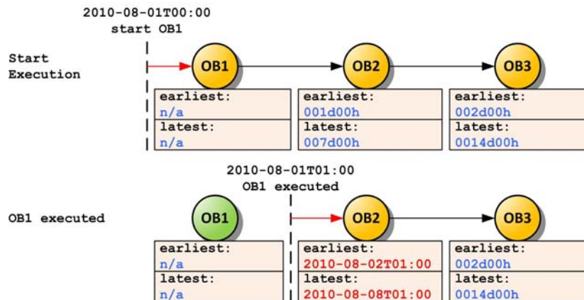
Figure 3. Execution of Time Link Container
