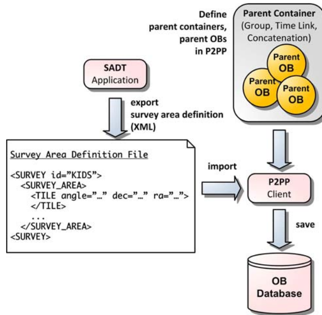
Figure 12. Definition of a Survey Area using SADT and import into P2PP
