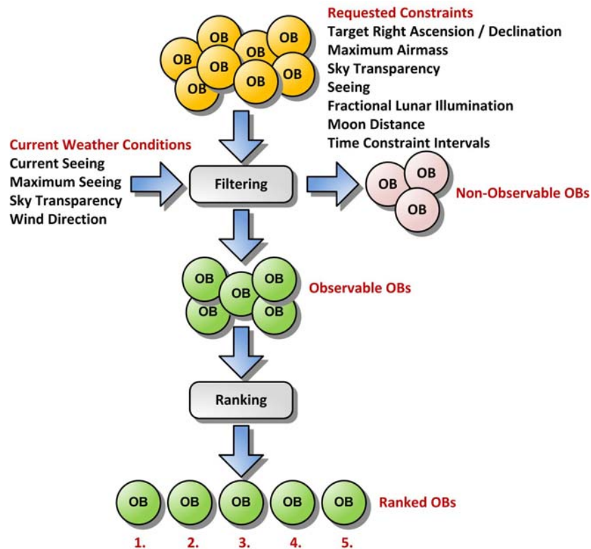
Figure 8. OB Filtering and Ranking
