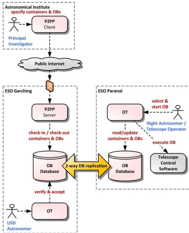
Figure 1. OB specification, review and execution workflow
