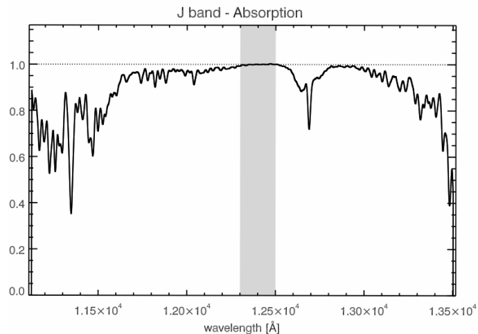
Figure 2: The J1.240 atmospheric window. Telluric absorption spectrum at R= 2000 as a continuous black line. The gray area shows the atmospheric window.
