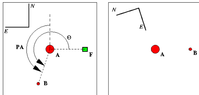
Figure 15: Setting the correct value of the TEL.ROT.OFFANGLE parameter. Left side: Object B located at a position angle PA = 162^\circ is to be brought at the apparent location F on the detector. Here, \Theta = PA + 90^\circ . Therefore, \text{TEL.ROT.OFFANGLE} = 360^\circ - \Theta = 108^\circ . Right side: Requested final orientation after completion of the telescope setup.
