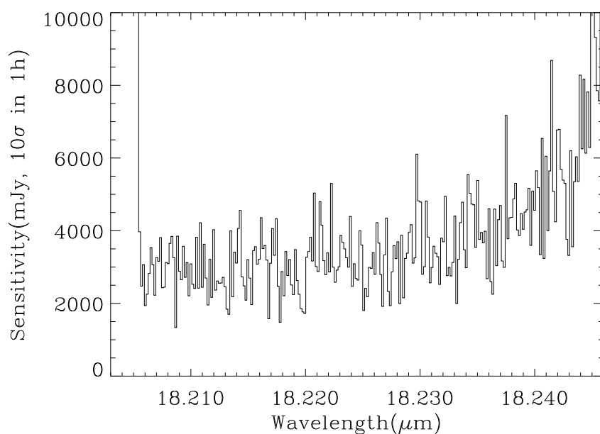
Figure 34: Observed sensitivity as a function of wavelength for high resolution mode. Offered sensitivity is typically a factor of 2 larger.
