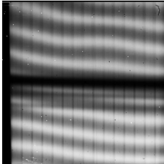
Figure 19: VISIR spectrum in staring, medium-resolution mode showing the detector fringing (white). The detector absorption feature at 8.8 \mu\text{m} is visible as black horizontal bar (cf. Fig. 8). Dark vertical stripes are caused by the non-uniform gain of the different electronic amplifiers. These features are largely removed by chopping.
