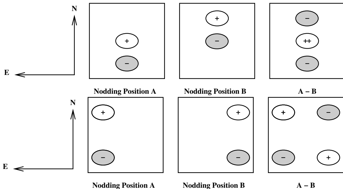
Figure 20: Schematic drawing of the content of a frame obtained with TEL.ROT.OFFANGLE = TEL.CHOP.POSANG = 0 and SEQ.CHOPNOD.DIR = PARALLEL (top) and SEQ.CHOPNOD.DIR=PERPENDICULAR (bottom). In the individual nodding positions, the positive beams correspond to the chopper position A and the negative beams to the chopper position B. Note that the default pointing position of the telescope corresponds to the center of the detector. Within the accuracy of the telescope pointing, this location matches the nodding position A, chopper position A if SEQ.CHOPNOD.DIR = PARALLEL .
