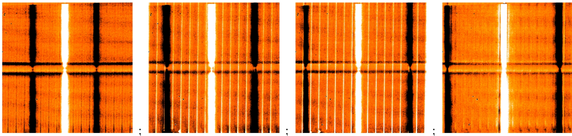
Figure 13: Sequence of chop/nod, reduced spectra obtained in the Medium Resolution mode with a central wavelength = 8.8\mu\text{m} . The TEL.CHOP.THROW = 8, 11, 13 and 14'' from left to right. Note the presence of significant striping when the 'left' beam hits some hot pixels at the lower left of the detector. For the location of the object along the slit (pixel X=123 at row Y = 128), this occurred for TEL.CHOP.THROW between 10 and 13'' , approximately. The horizontal lines at the middle of the images are caused by the lack of detector response at 8.8\mu\text{m} .
