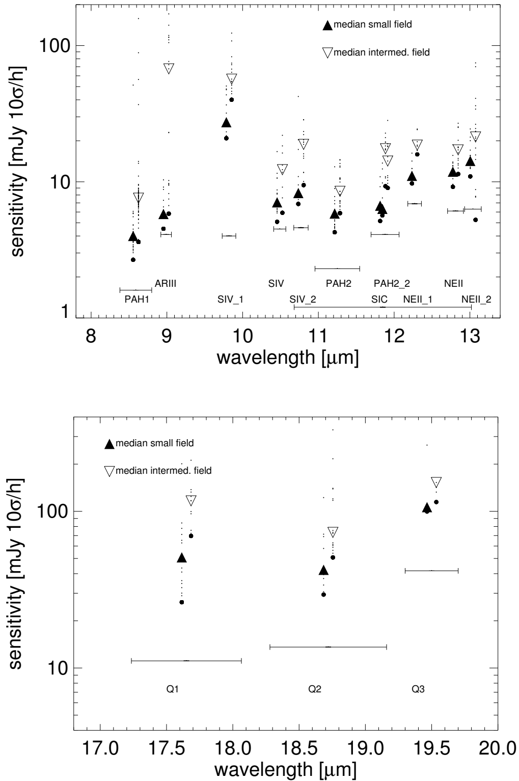
Figure 4: Sensitivities for the VISIR imager for the N (top) and Q-band (bottom). Small and intermediate field observations are displaced for clarity. Background noise limits are indicated for the individual filter bandpasses.
