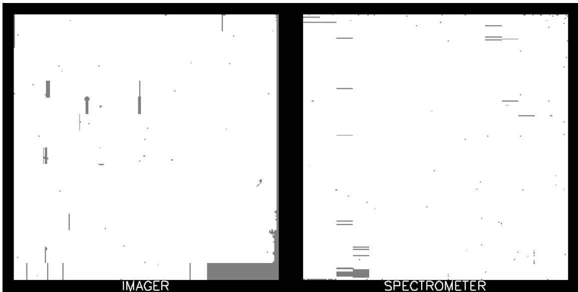
Figure 11: Bad pixel maps of the imager (left) and spectrometer (right) detectors. The large grey rectangular areas correspond to electronically masked pixels in order to decrease detector striping.
