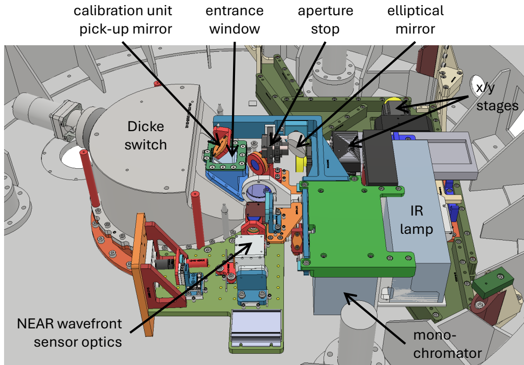
Figure 12: Schematic drawing of the VISIR Flange Module on top of the VISIR cryogenic vessel.
