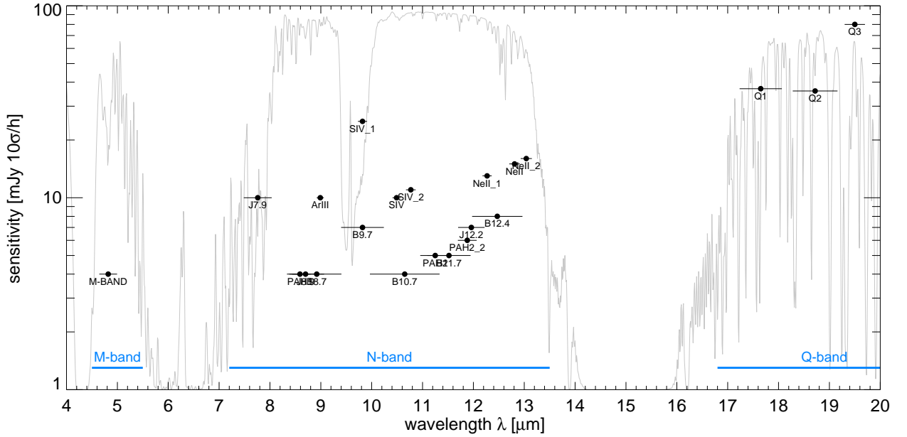
Figure 6: Offered sensitivities for the various filters of the VISIR imager in the M-, N- and Q-bands as a function of the filter wavelength and width. The atmospheric transparency spectrum for PWV = 1 mm at an airmass of 1 is plotted in the background.
