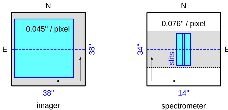
Figure 17: Field orientation and pixel scale for the imaging (SF) and the spectroscopic modes of VISIR for TEL.ROT.OFFANGLE = 0° . While the imaging detector follows the normal astronomical convention, the spectroscopic detector is reversed in x -direction so that East is to the right. The gray area marks the region of the detector which is typically read-out, the spectroscopy detector being windowed in y -direction. The magenta areas mark the areas illuminated by the sky – in case of the spectrometer for the very wide slit (“OPEN”). The sizes of these usable areas on sky are given in blue (see also § 3.4).
