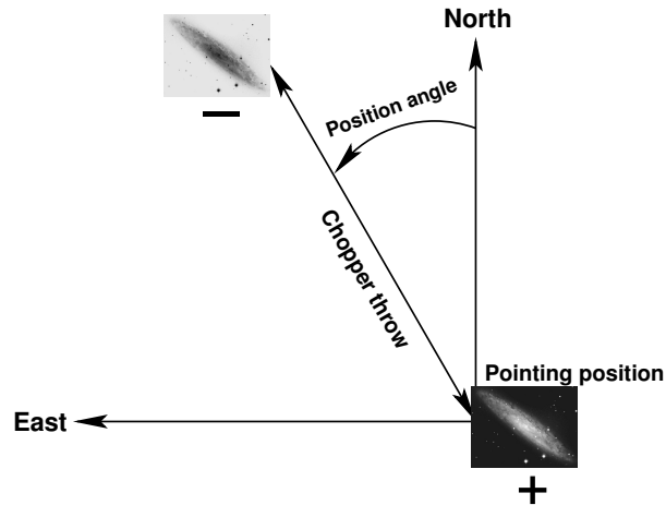
Figure 18: Definition of chopping parameters from the telescope point-of-view. The (chopping) position angle ( TEL.CHOP.POSANG ) is measured counter-clockwise from North to East, between 0^\circ and 360^\circ . The positive beam (+) is obtained when the M2 is at Chopping Position A and corresponds to the pointing position of the telescope as given in the FITS header (idle position). The negative beam (-) is obtained by moving the M2 so that it points to a position angle on the sky given by TEL.CHOP.POSANG and a throw of TEL.CHOP.THROW from the telescope pointing position (Chopping Position B). If TEL.CHOP.POSANG = TEL.ROT.OFFANGLE , the resulting image on the detector will appear as in one of the nodding position images illustrated in Fig. 20.
