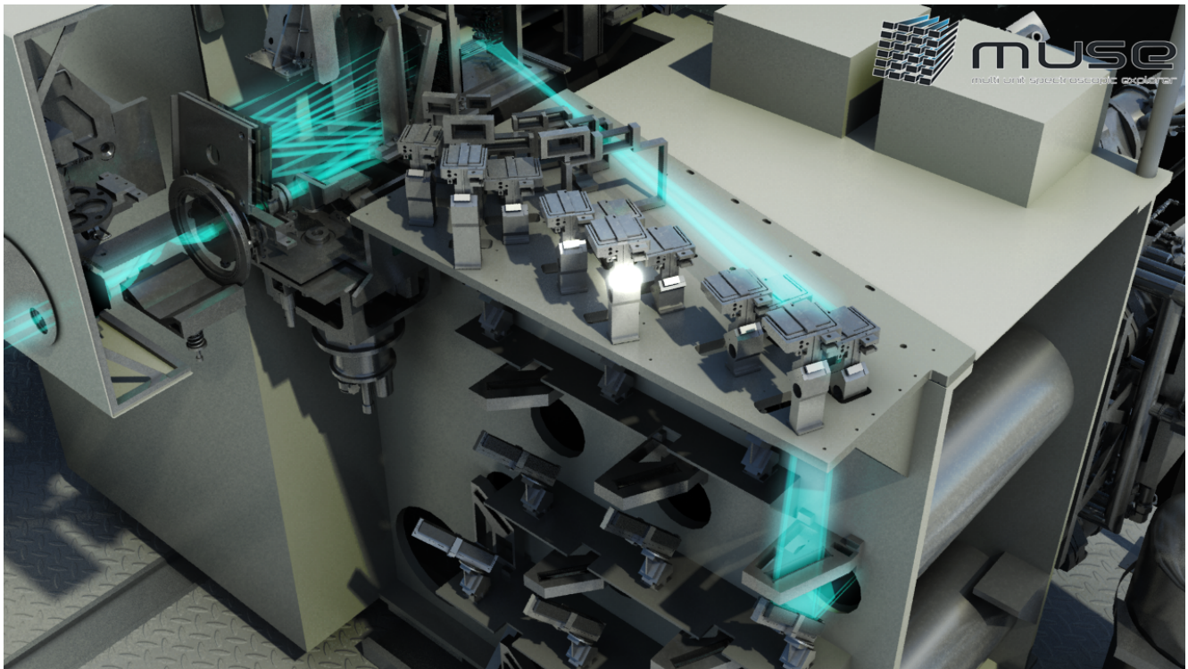
Figure 6: 3D view of optical paths for all channels due to the relay optics splitting of the field-of-view into 24 channels. The bottom figure shows the path of lightrays for one of the channels, as seen from the Fore-Optics
