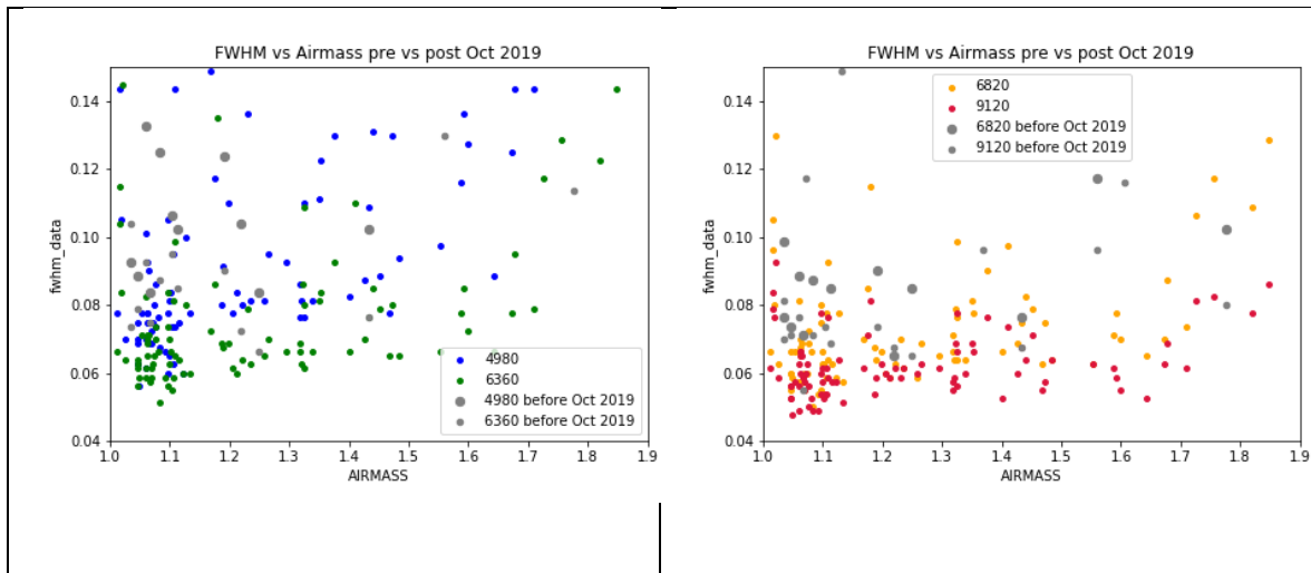
Figure 33 FWHM of the core of the NFM PSF for different airmasses before the 2019 campaign, grey, and after the campaign, in color, for selected wavelengths as indicated in the legends.
