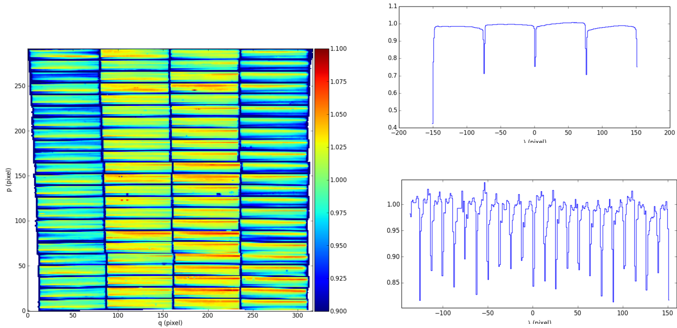
Figure 19: (left) normalized reconstructed image of the continuum flat-field in WFM. (right) horizontal (top) and vertical (bottom) cuts through the normalized image showing the horizontal and vertical variations in illumination.
