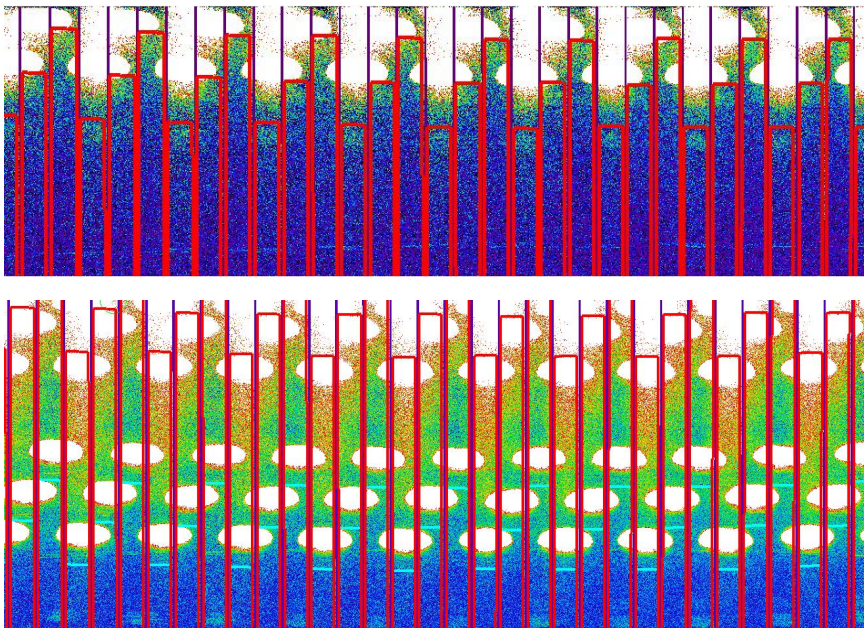
Figure 13: Second order effect in nominal (top panel) and extended (bottom panel) modes, shown here for a bright exposure with arc lines. The red boxes mark the slice limits up to 930 nm. The impact of second order is visible as the white ellipses illuminating the top of the detector. The nominal instrument mode is not affected by contamination, but it is more significant in the extended instrument mode.
