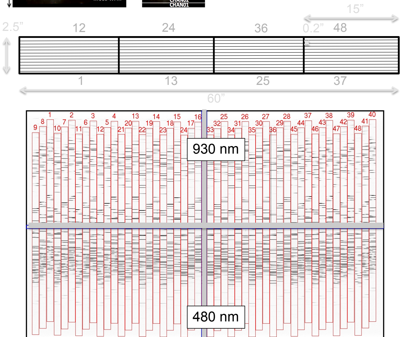
Figure 9: Overview of the splitting of the field-of-view from the fore-optics to one of the MUSE detectors. Left: splitting of the MUSE FOV into 24 sub-fields entering each channel. Center: shape of the entrance slicer on sky, with 4 stacks of 12 slices (numbered in red from 1 to 48) covering a 2.5 x 60" field. Bottom: location of each slice on the detector, with the corresponding wavelength range.
