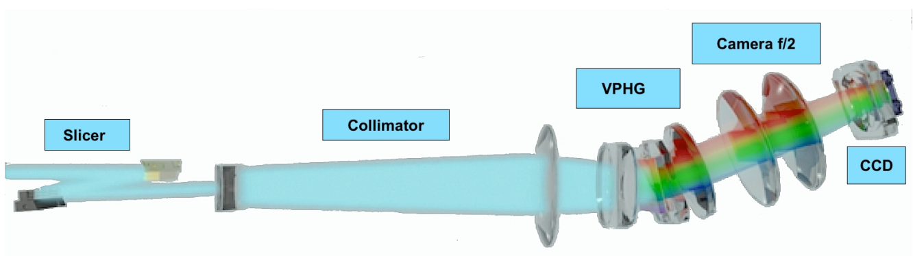
Figure 7: Overview of the optical layout for one of the IFUs. The top panel shows one of the slicers, which cuts the FOV of each channel into 4 stacks of 12 slices. The bottom panel shows the optical elements in the IFU and the path of light to the CCD.
