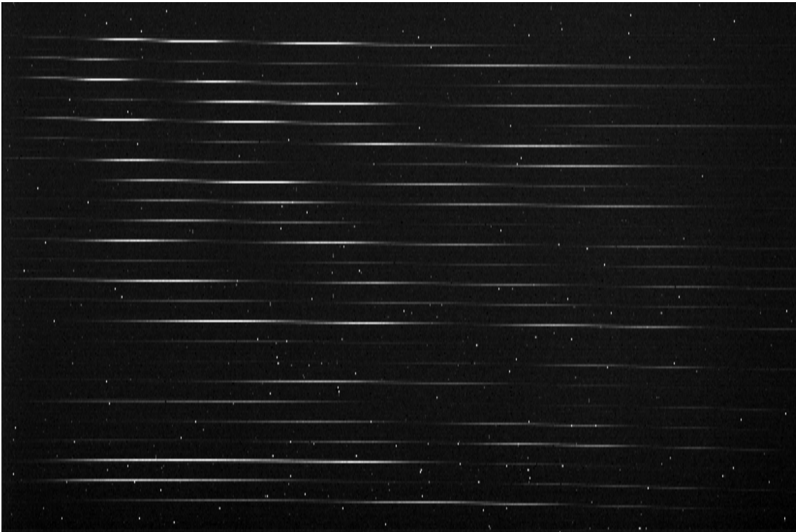
Figure 1: One raw Gravity frame on the science channel. Wavelength runs horizontally. In contrast to other beam combiners, Gravity does not record entire fringe packets but only four points on the central fringe (i.e. the so-called ABCD method of fringe detection). For each polarization, each pair of telescopes yields thus 4 spectra. The fringe can be seen by comparing spectra pertaining to the same pair of telescopes. The total number of spectra is thus 24: 6 pairs of telescopes, 4 points ( viz. A,B,C,D) per pair.
