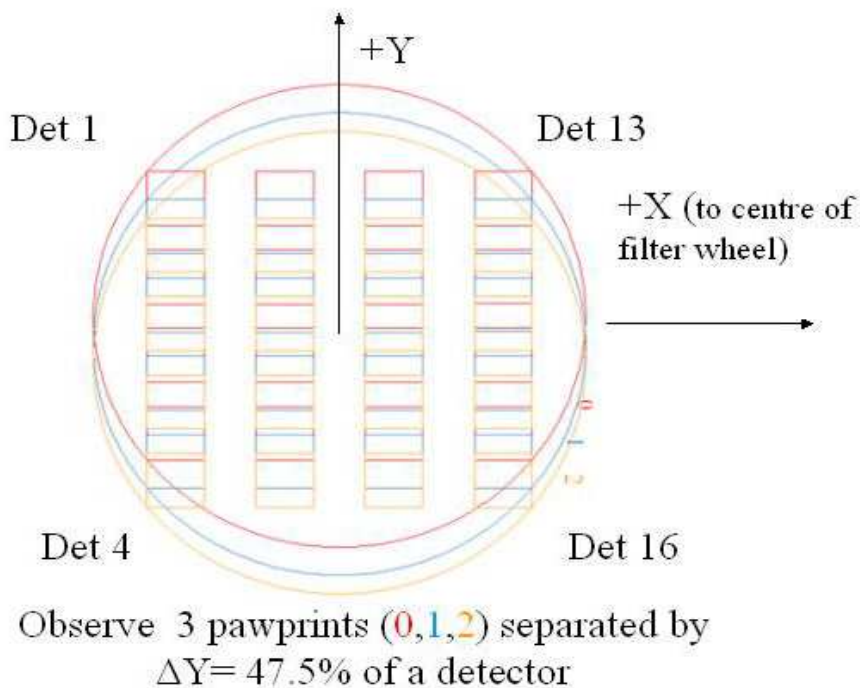
Figure 17: Completing a tile with six pawprints: the three vertical steps along the Y axis.
