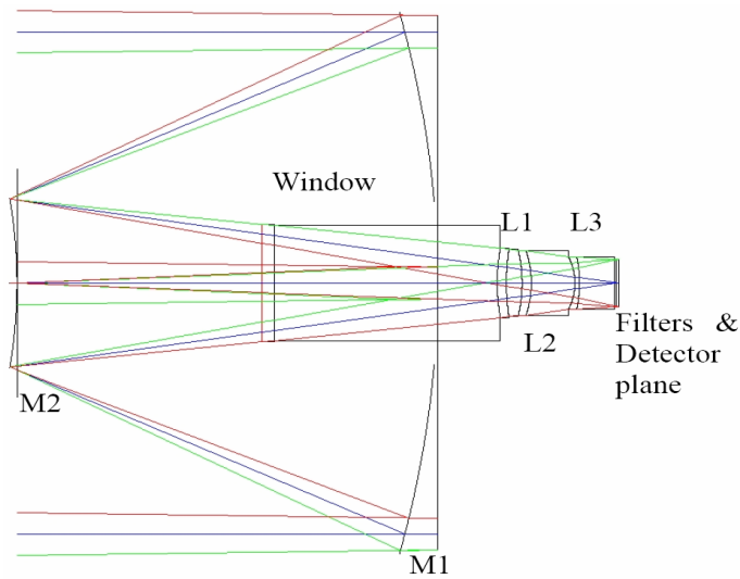
Figure 2: Optical layout of the telescope. M1 and M2 are the telescope primary and secondary mirrors. The camera's entrance window, the three lenses L1, L2, and L3, the filter and the detector planes are also marked.
