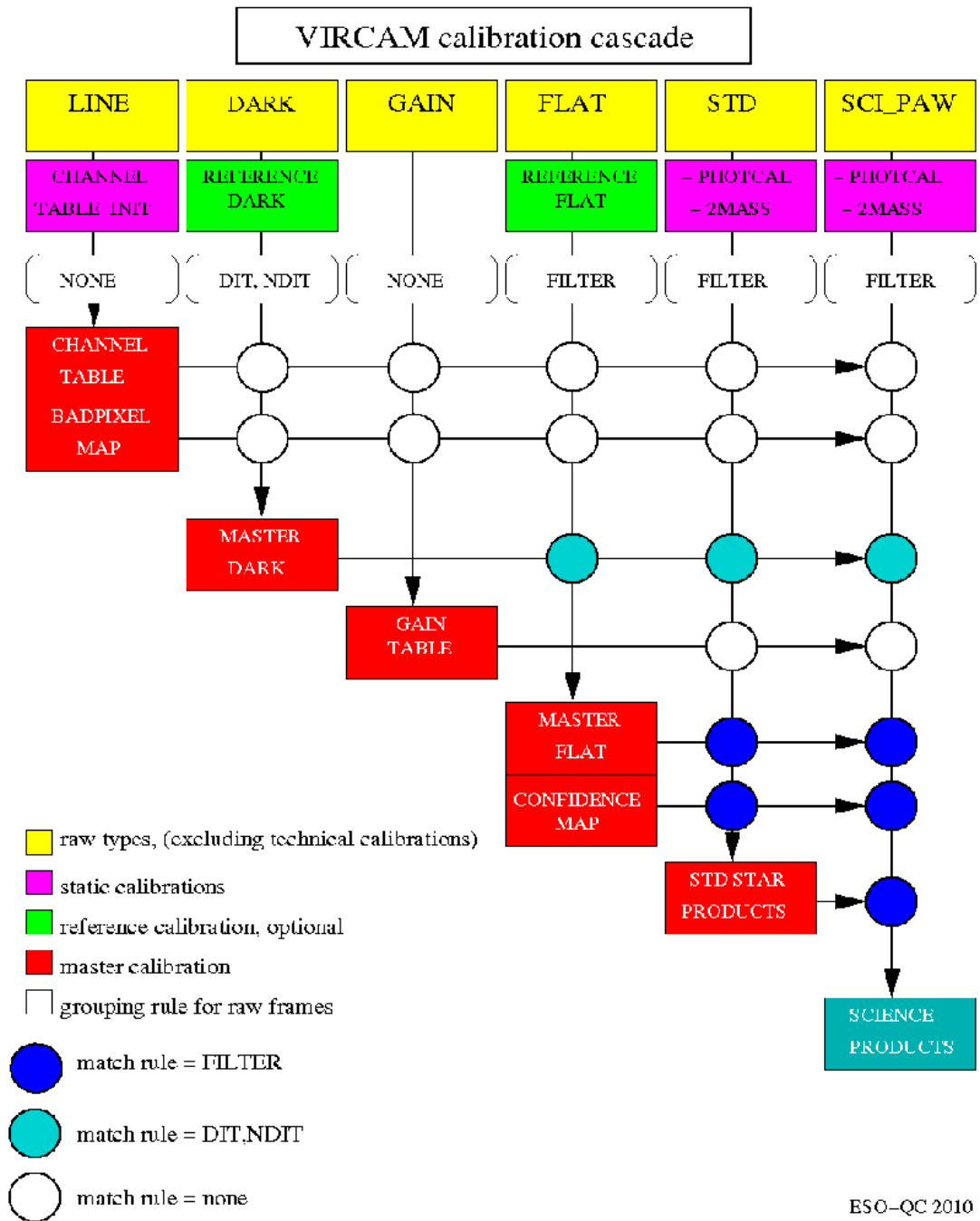
Figure 19: VIRCAM cascade diagram for producing calibration frames.
