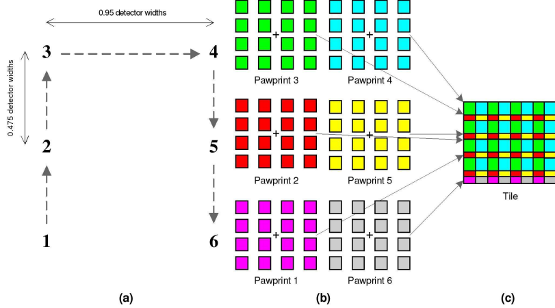
Figure 16: Contiguous tile, formed by combination of six overlapping pawprints.
