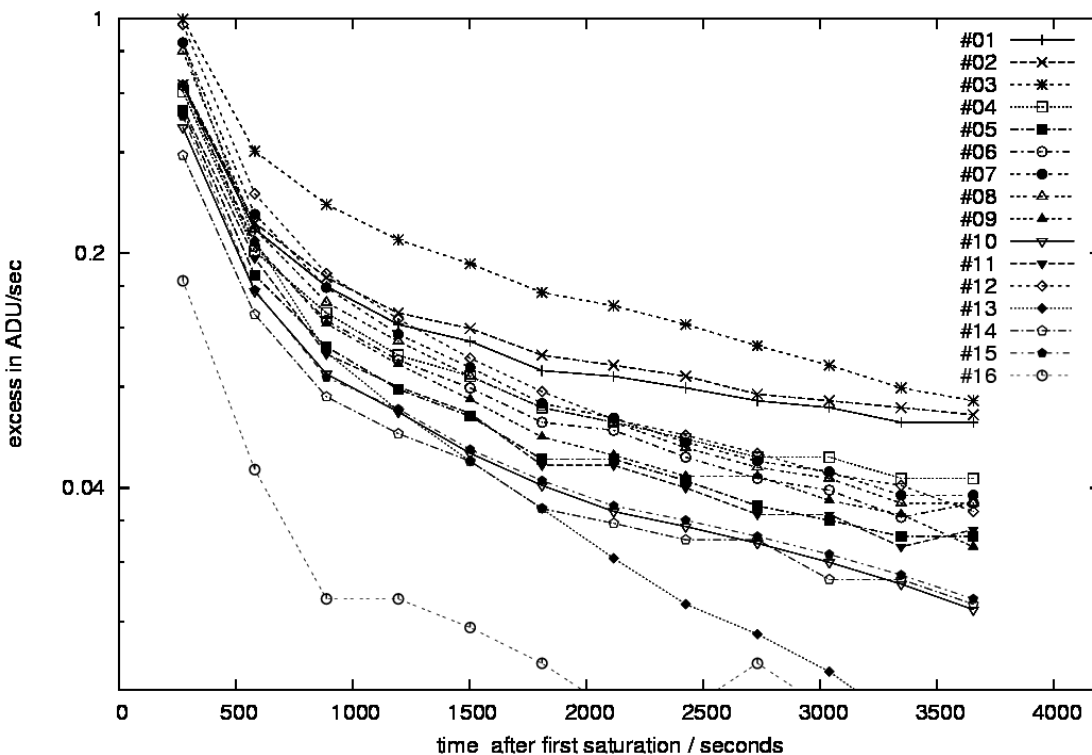
Figure 7: VIRCAM persistence for the individual detectors.
