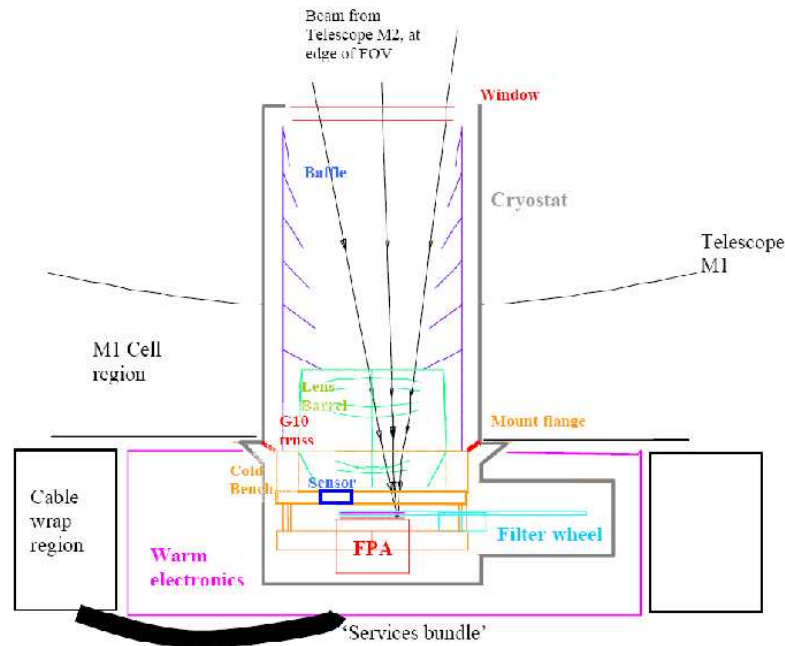
Figure 4: VIRCAM optical layout.
