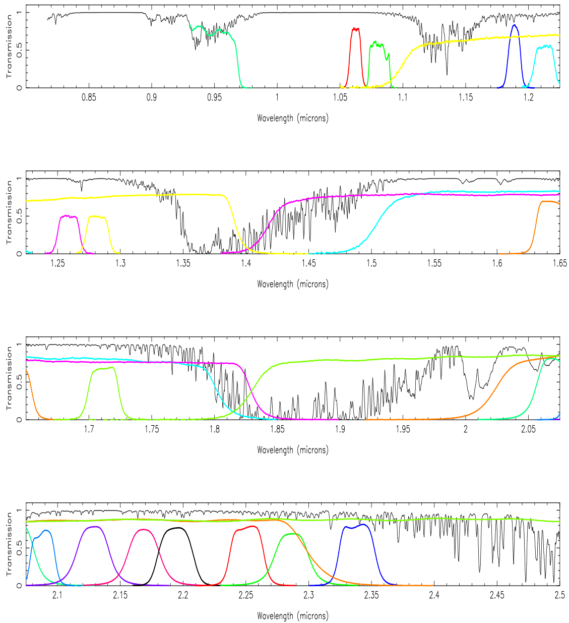
Figure B.1: The atmospheric transmission at a resolution of 8Å.
