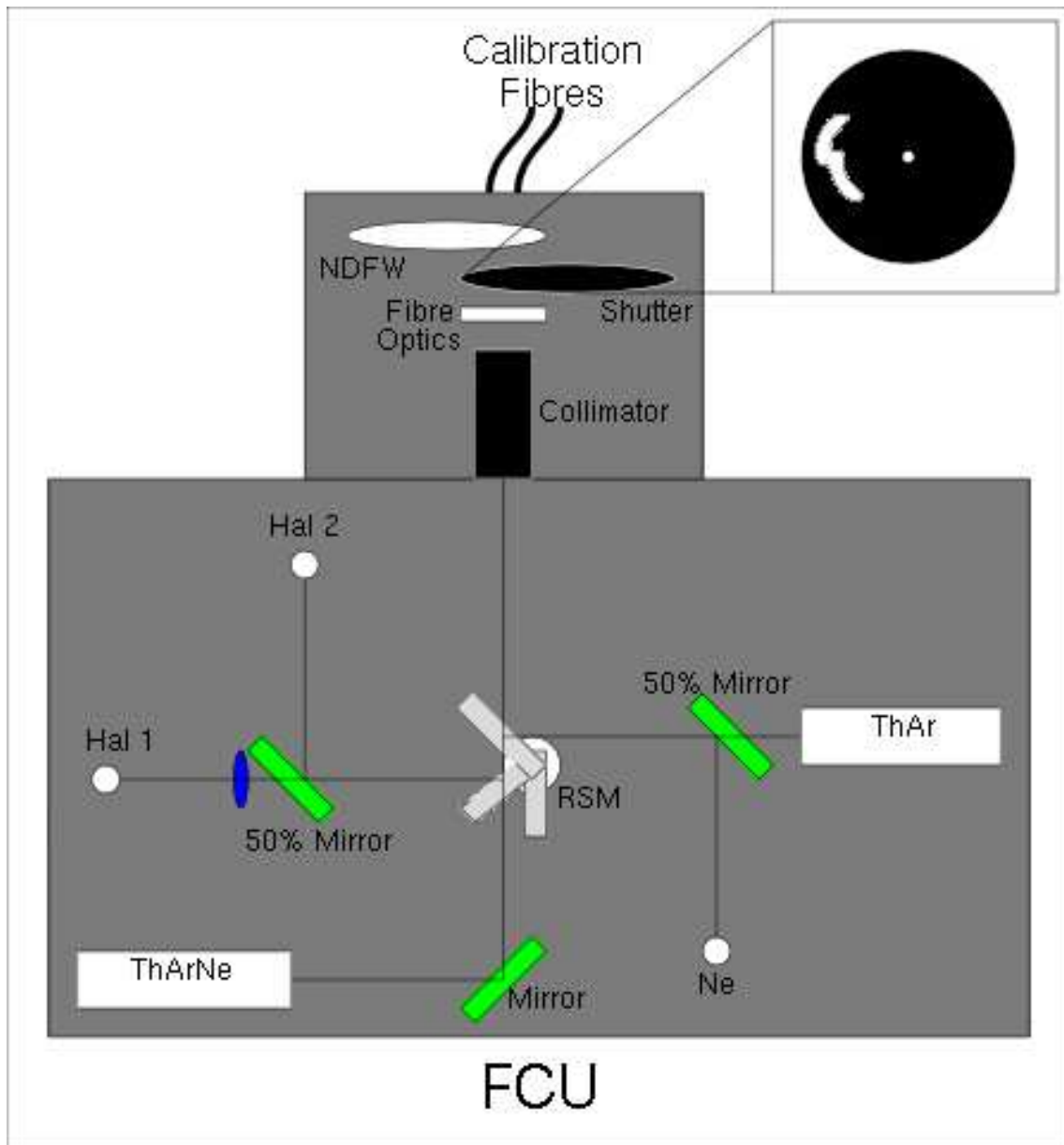
Figure 2.3: Schematic diagram of the FCU.
