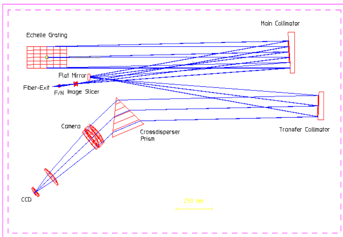
Figure 1.1: FEROS optical system from fibre exits to detector.
