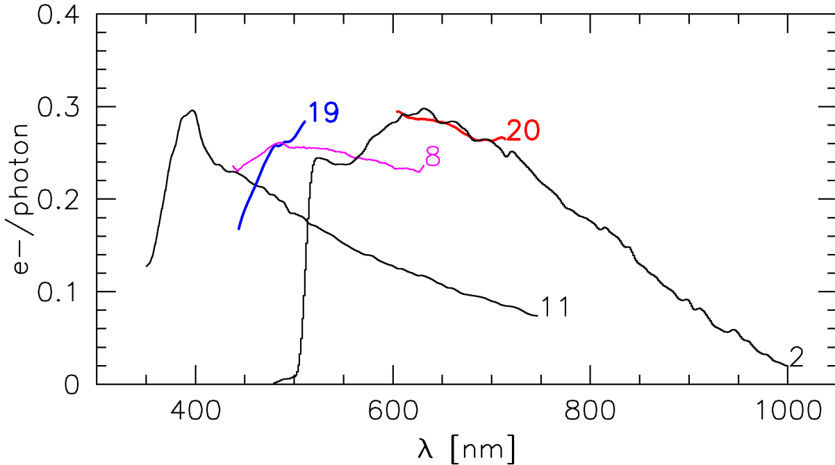
Figure 7: System efficiency given by VPHGs #19 (blue curve) and #20 (red curve) compared to that of other EFOSC2 gratings.
