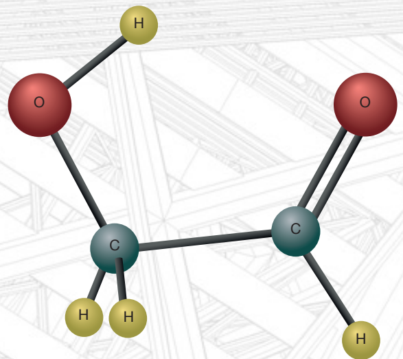
Glycolaldehyde
