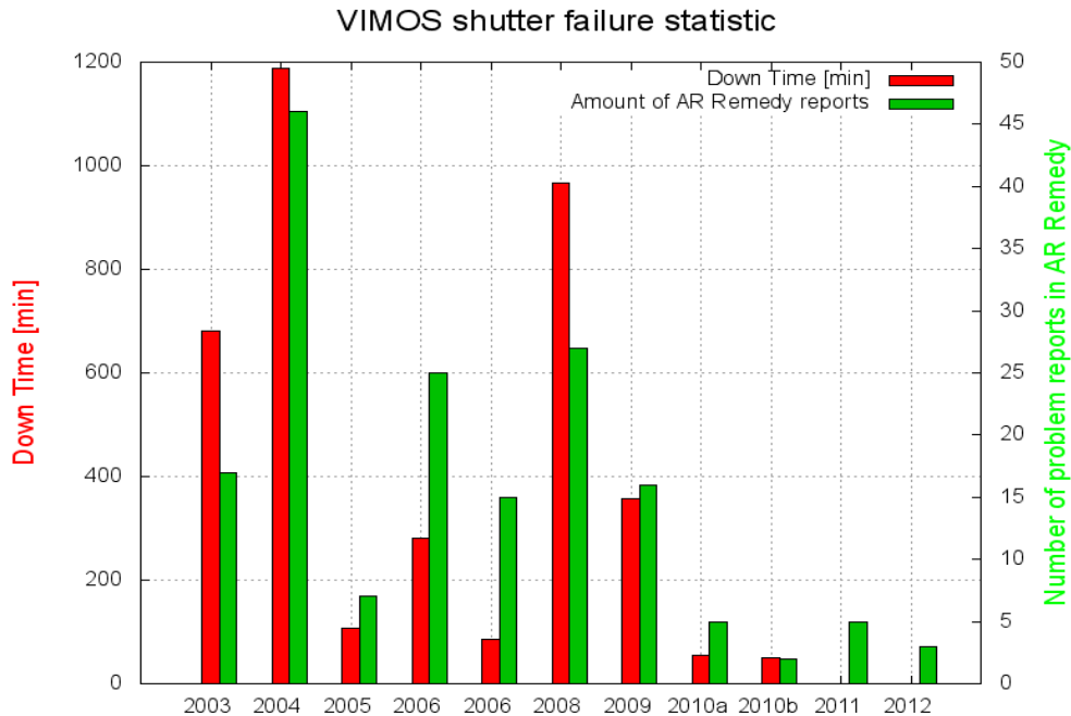
Figure 10: Shutter reliability
