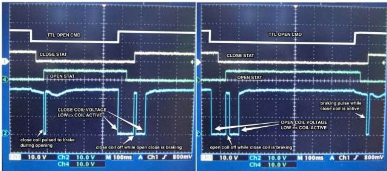
Figure 9: SDCU coil and status signal for braking mode
